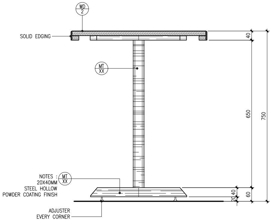
DINING TABLE - SECT 3
