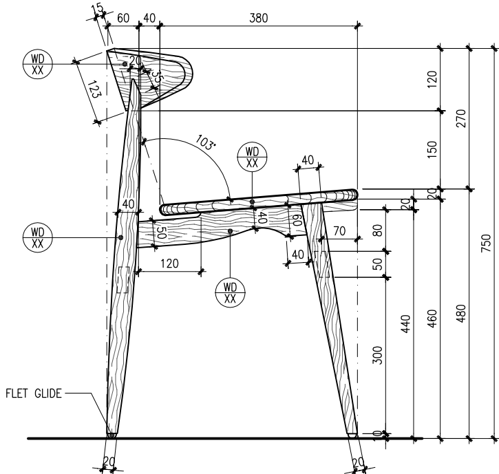
DINING CHAIR - ELEV
