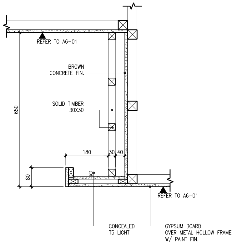
CEILING DETAIL 1 1 : 10 0 10 20 Cm
