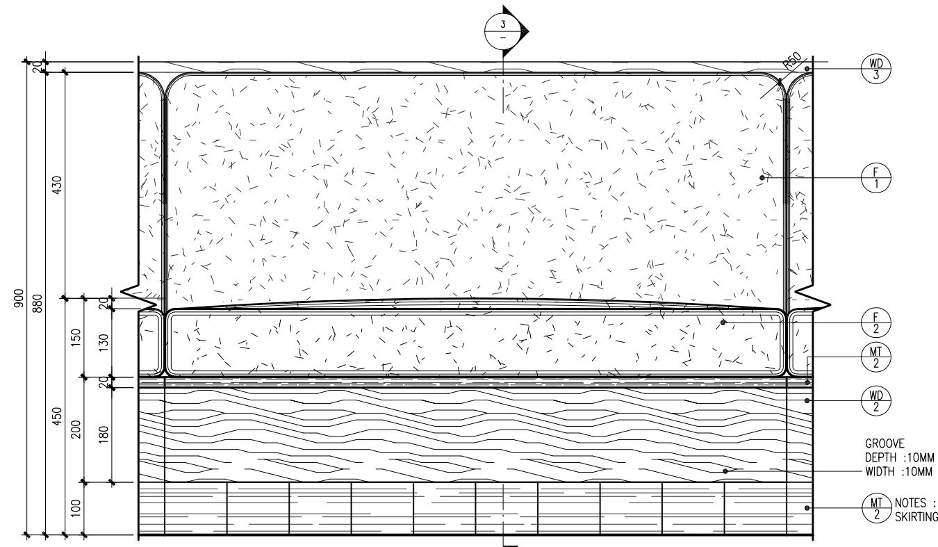
BANQUETTE SEATING - ELEV. 2
