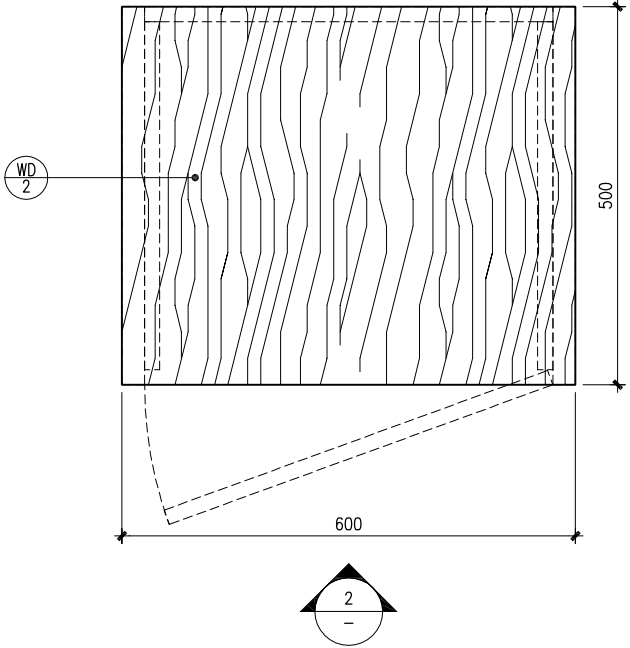
WAITER STATION TYPE 2&3 - PLAN 1
