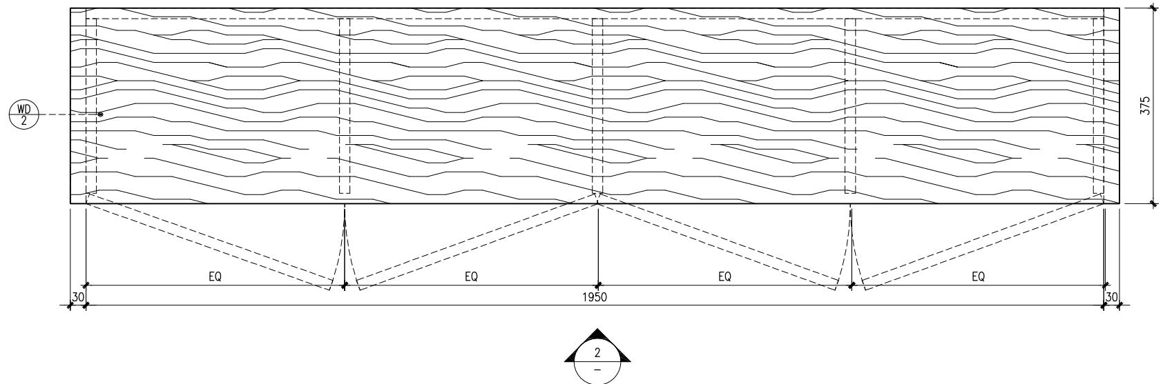
WAITER STATION TYPE 1- PLAN 1 1 : 10 0 10 20 Cm
