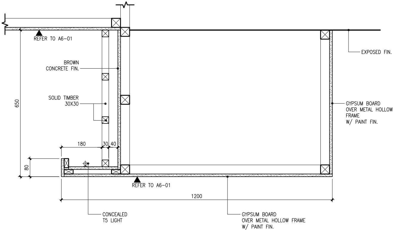
CEILING DETAIL 2 1 : 10 0 10 20 Cm
