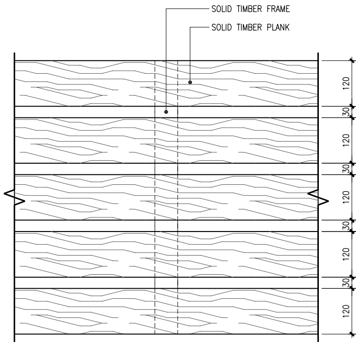
CEILING DETAIL 3 1 : 10 0 10 20 Cm
