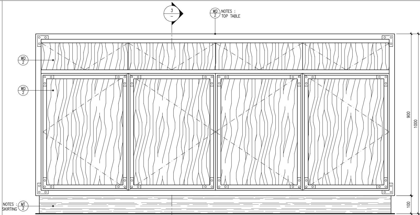
WAITER STATION TYPE 1- ELEV. 2 1 : 10 0 10 20 Cm
