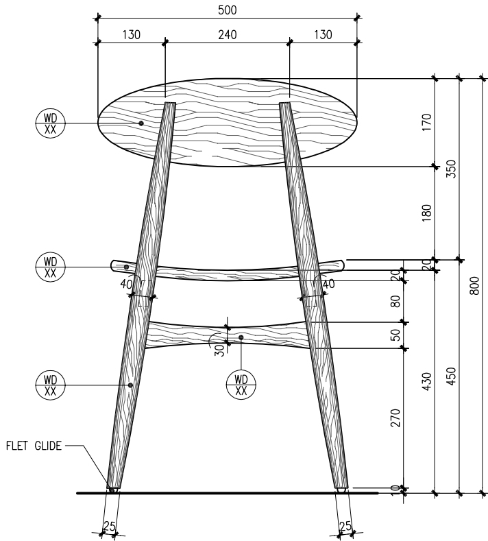
DINING CHAIR - ELEV
