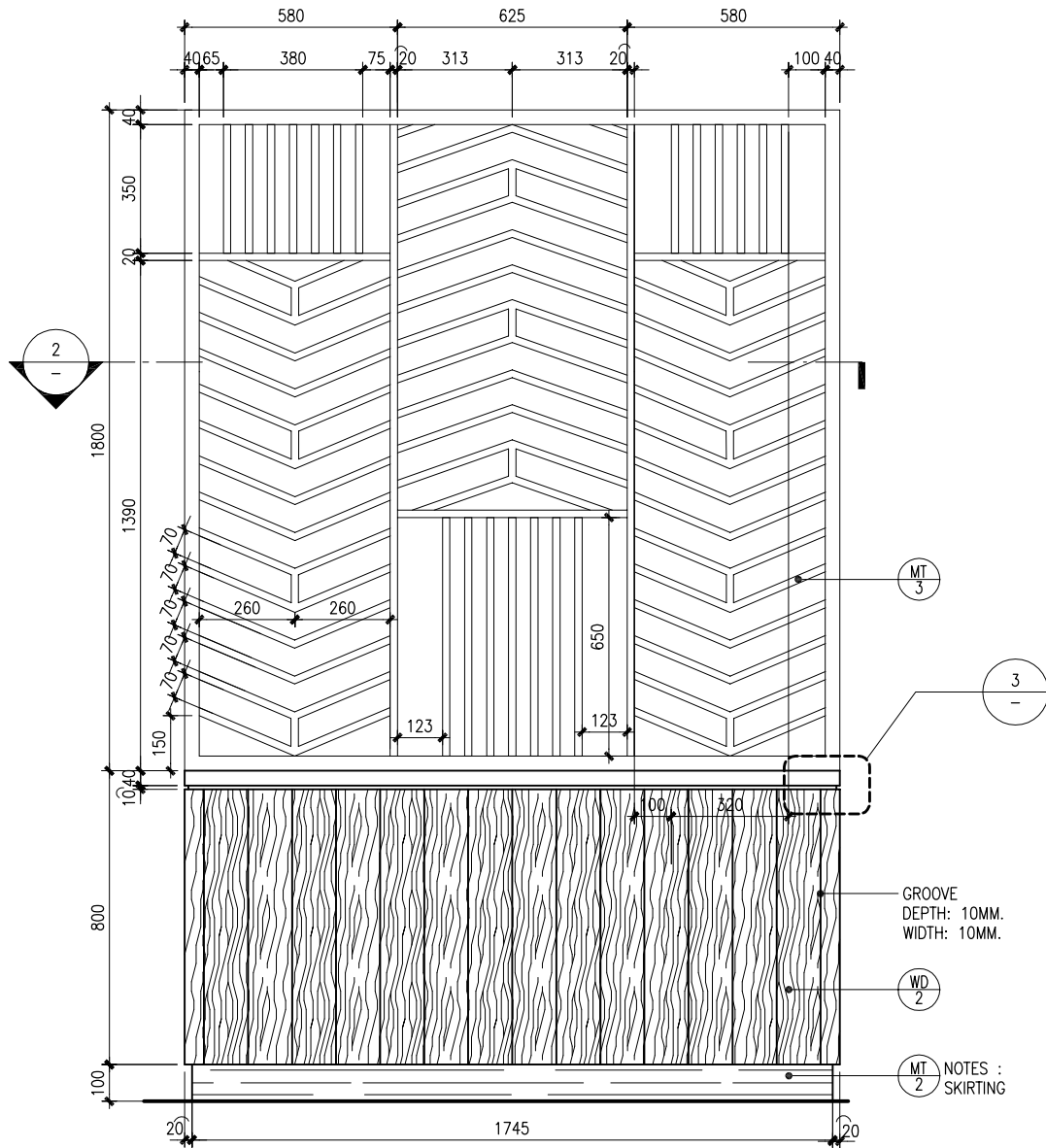
PARTITION DETAIL-ELEV.
