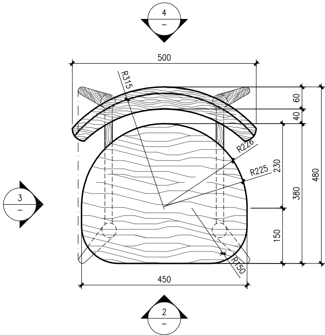
DINING CHAIR - PLAN
