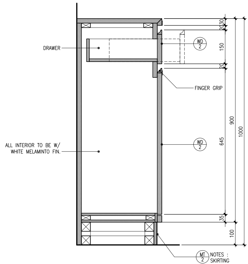
WAITER STATION TYPE 1- ELEV. 3 1 : 10 0 10 20 Cm
