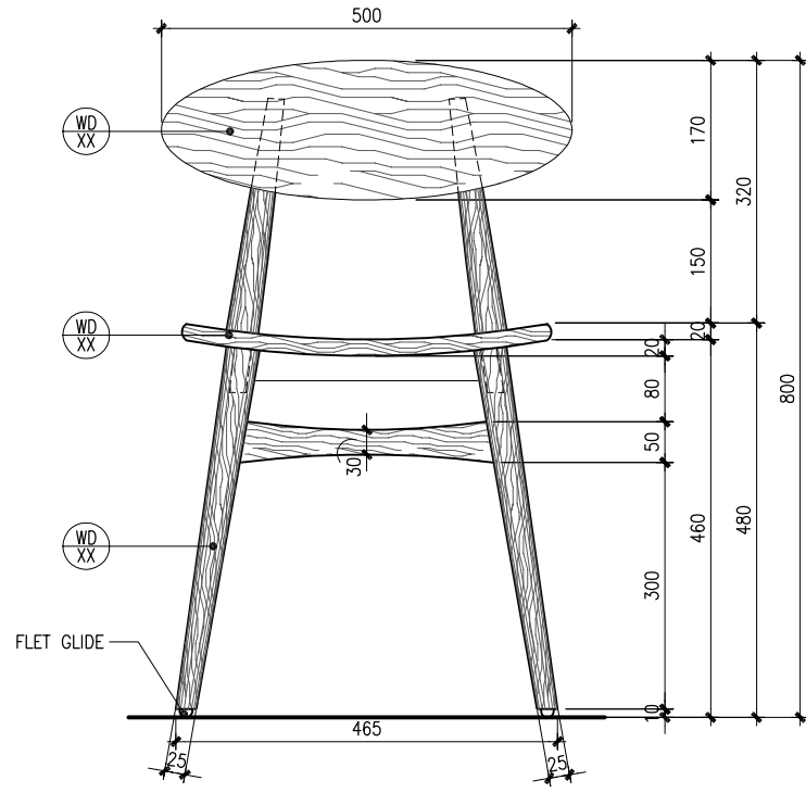
DINING CHAIR - ELEV
